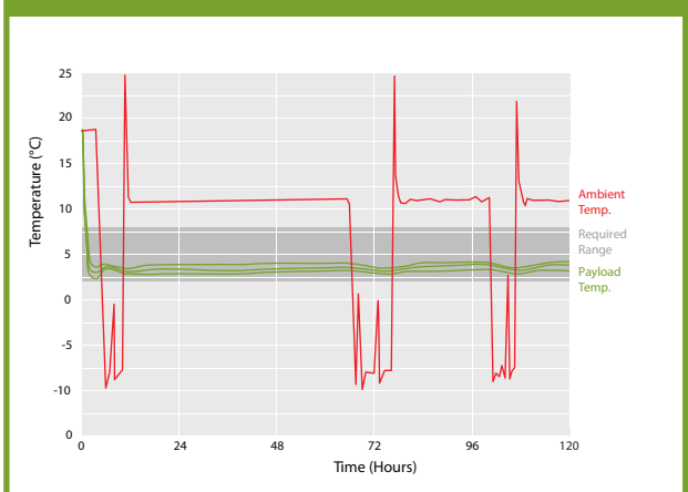
WINTER: 2°C to 8°C (Payload = Air)
