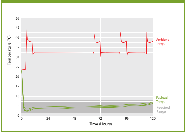
SUMMER: 2°C to 8°C (Payload = Air)
